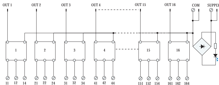
SCHEMA A BLOCCHI MODULI 8-12-16 USCITE 8-12-16 OUTPUT MODULES BLOCK DIAGRAMS
